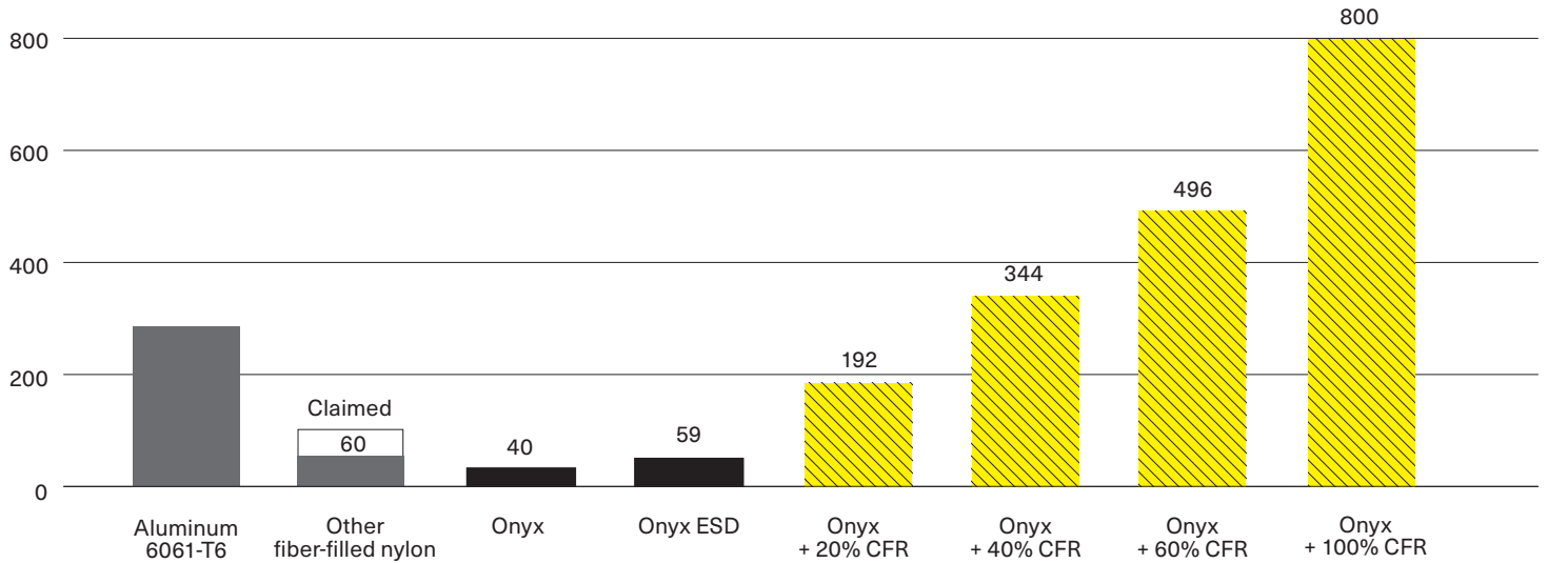
Tensile Strength (MPa) Conditioned to ASTM D638 Specifications
